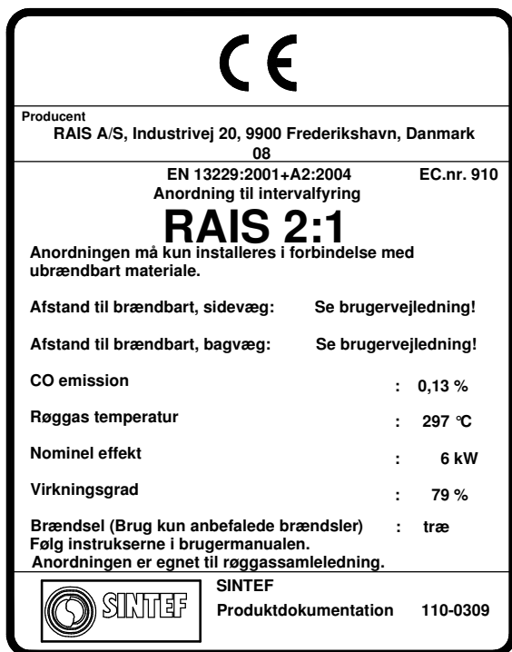
Manufacturer's Plate for RAIS 2:1
